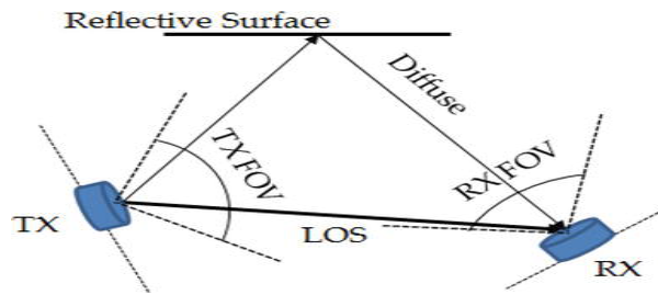
Figure 3: Schematic view of LOS and diffuse OWC links.
