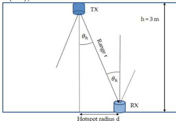
Figure 9 Geometry of the worst case hotspot alignment.
