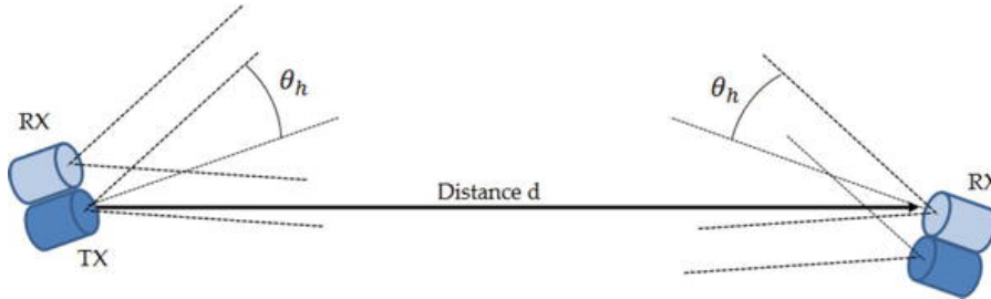
Figure 7 Point and shoot configuration.
