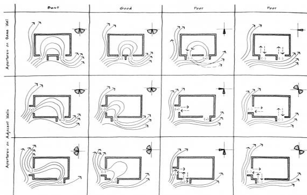
Fig. 1.3: Different wing walls of better and worse effectiveness, on same wall and adjacent walls. Source: DeKay and Brown (2001)
