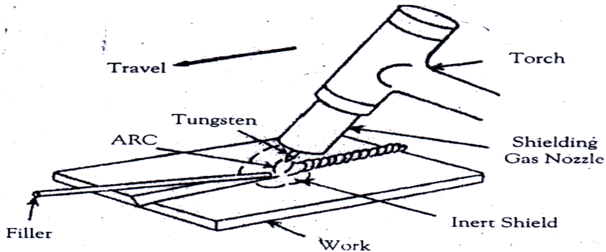
Figure 2.18: Gas tungsten arc welding Source: Ashutosh (2020)
